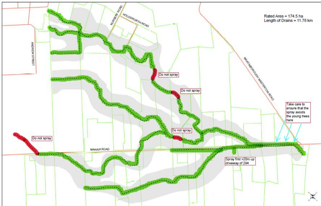
Manaia Drainage Scheme
